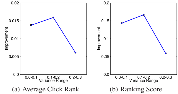
Figure 4: Improvement vs. variance in S_c .
