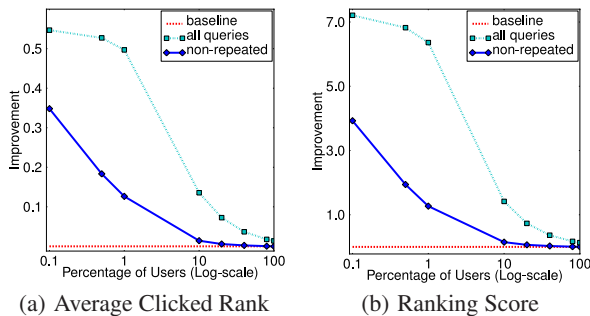
Figure 2: Improvement over baseline: computed on all queries and on non-repeated queries only.
