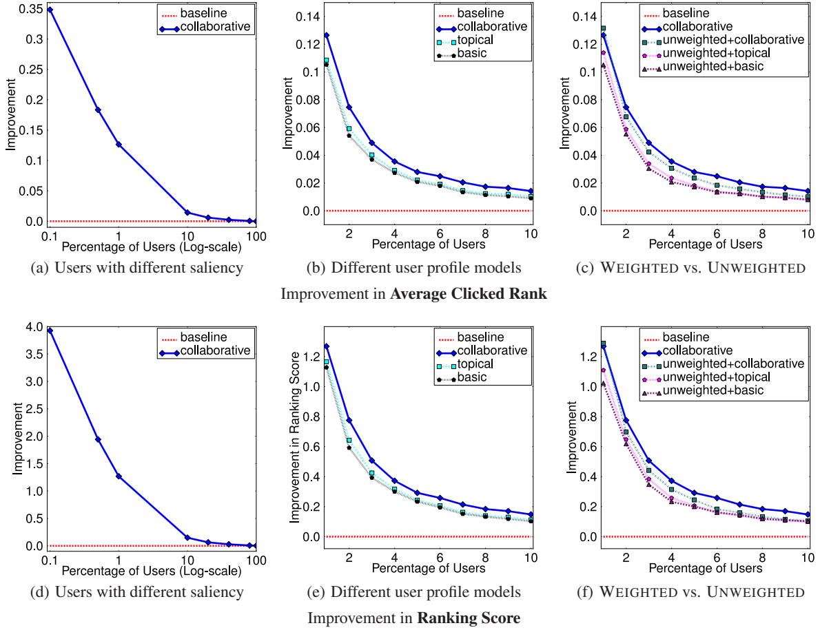
Figure 3: Performance analysis focusing on high- Q_u users: comparing WEIGHTED-LCAA + COLLABORATIVE with its variations.
